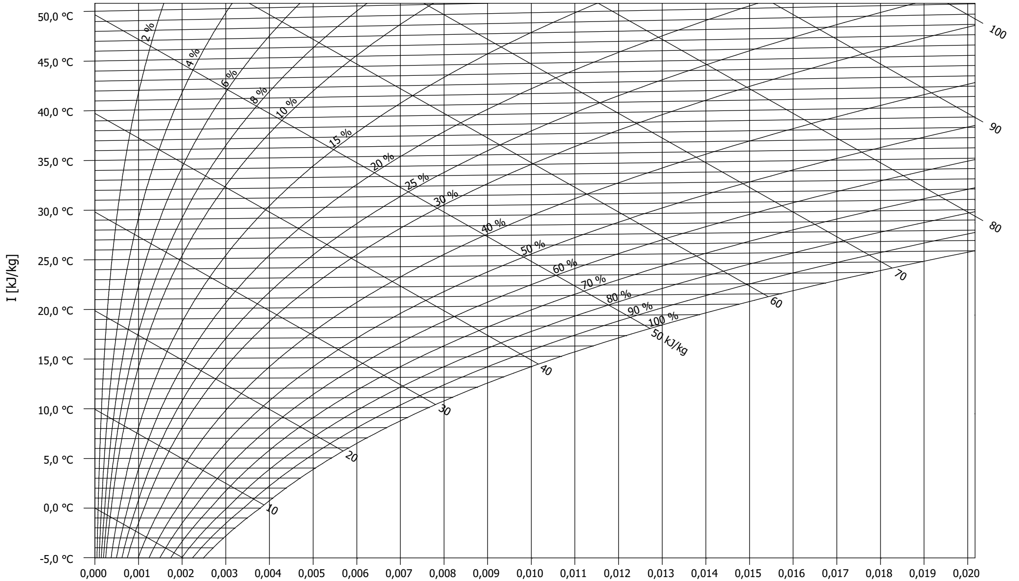
IX Diagram for moist air in the temperature range -5 °C to +50 °C (h=1013 mbar)
